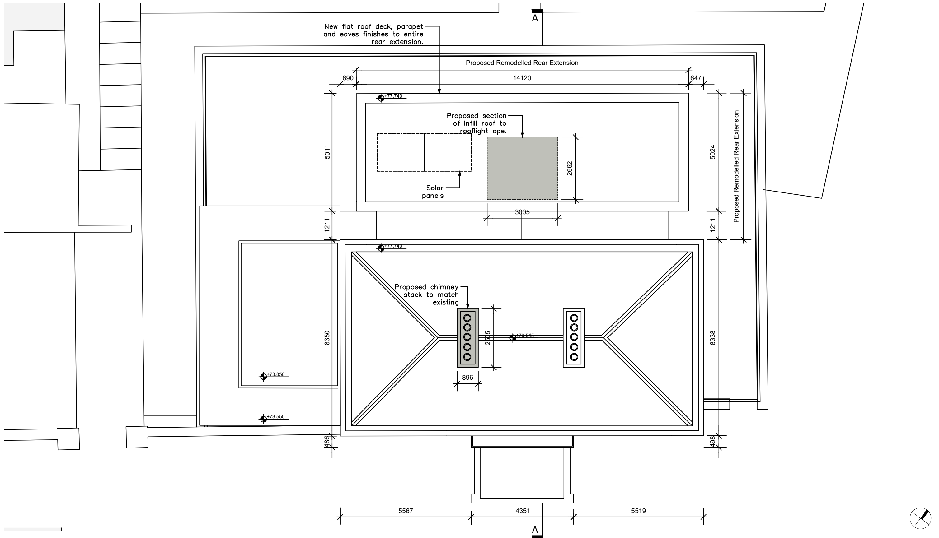
Cedar Mount House, Proposed Roof Plan
